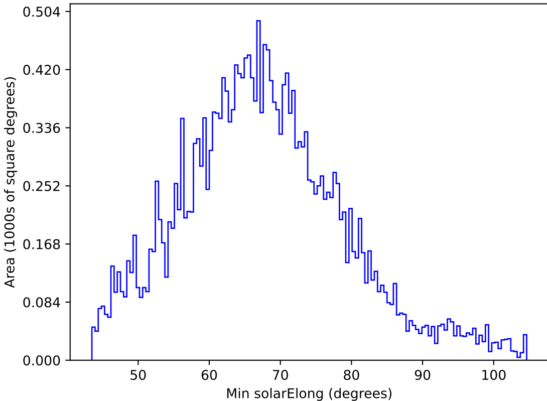
too_5_4v3.4_10yrs All sky y band: Min solarElong
