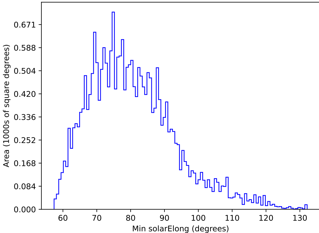
too_5_4v3.4_10yrs All sky u band: Min solarElong
