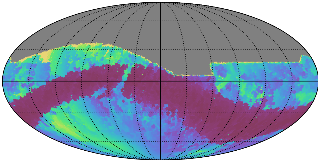
too_5_4v3.4_10yrs All sky r band: Min solarElong
