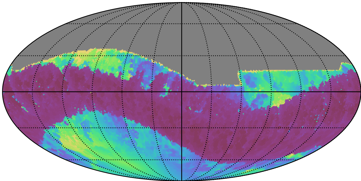
too_5_4v3.4_10yrs All sky i band: Min solarElong
