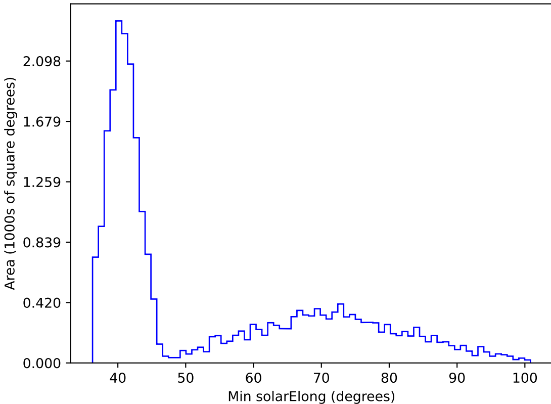
too_5_4v3.4_10yrs All sky i band: Min solarElong
