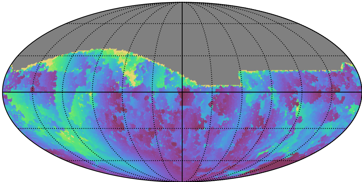
too_5_4v3.4_10yrs All sky g band: Min solarElong
