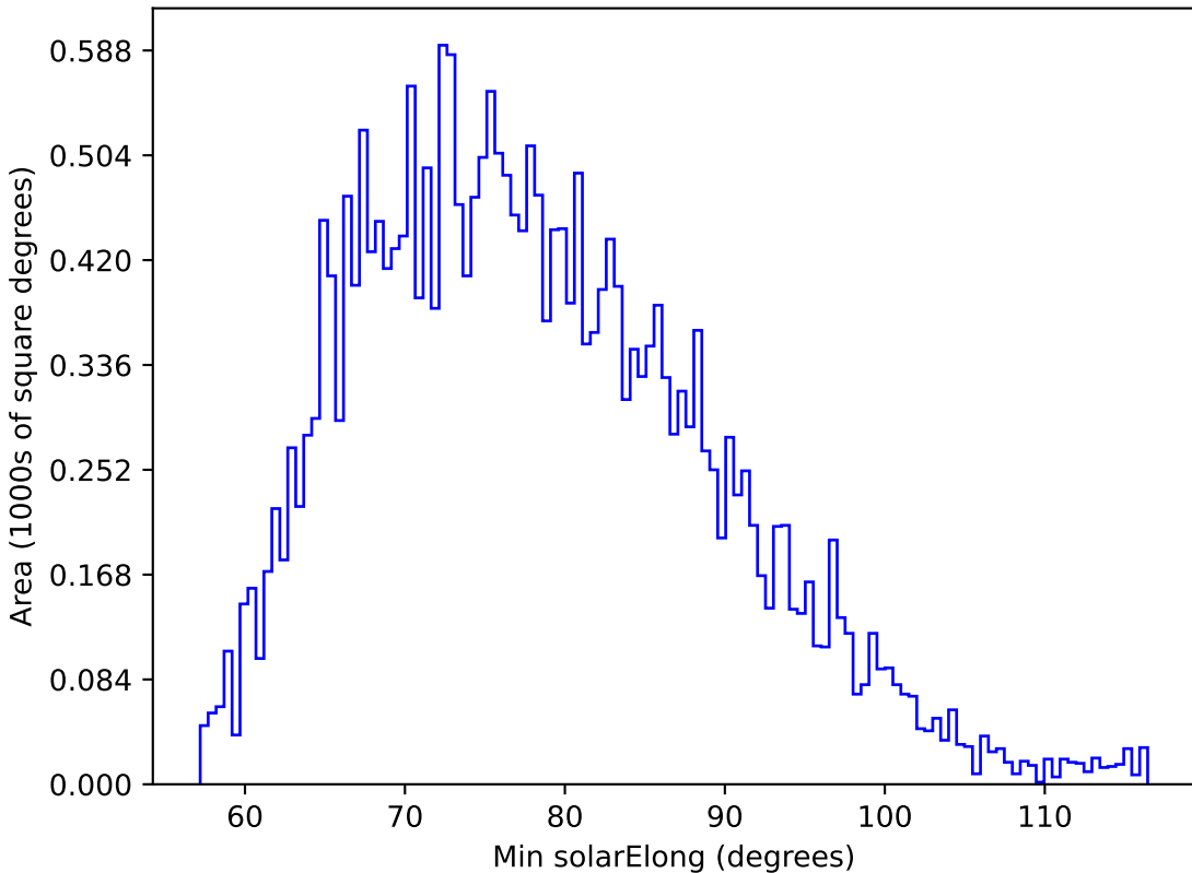
too_5_4v3.4_10yrs All sky g band: Min solarElong
