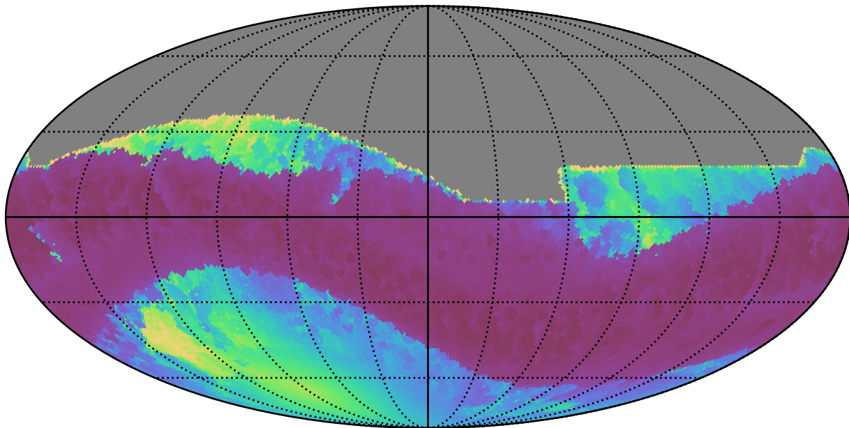
too_5_4v3.4_10yrs All sky all bands: Min solarElong
