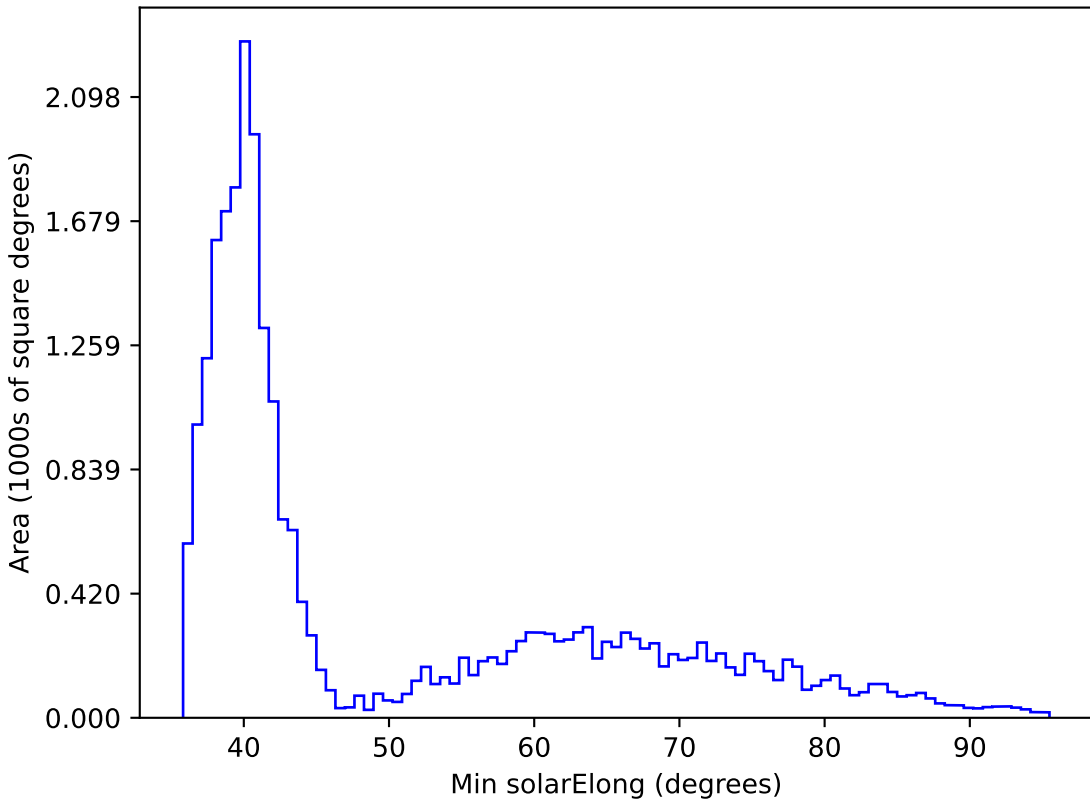
too_5_4v3.4_10yrs All sky all bands: Min solarElong
