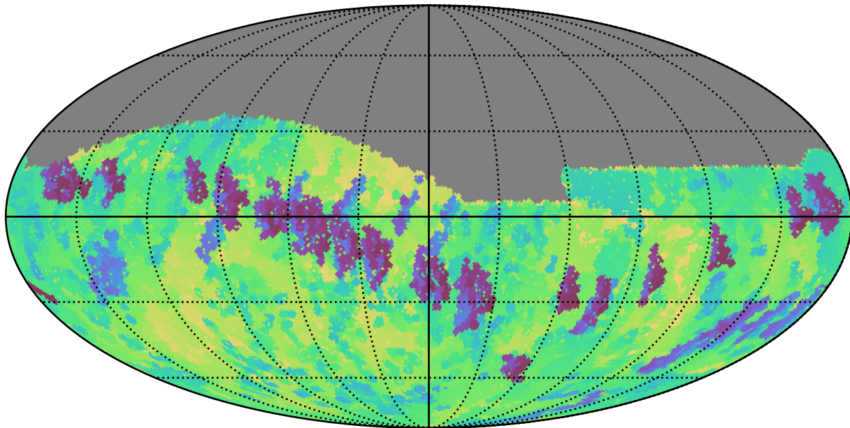
too_5_4v3.4_10yrs Yr 1 z band: Min skyBrightness
