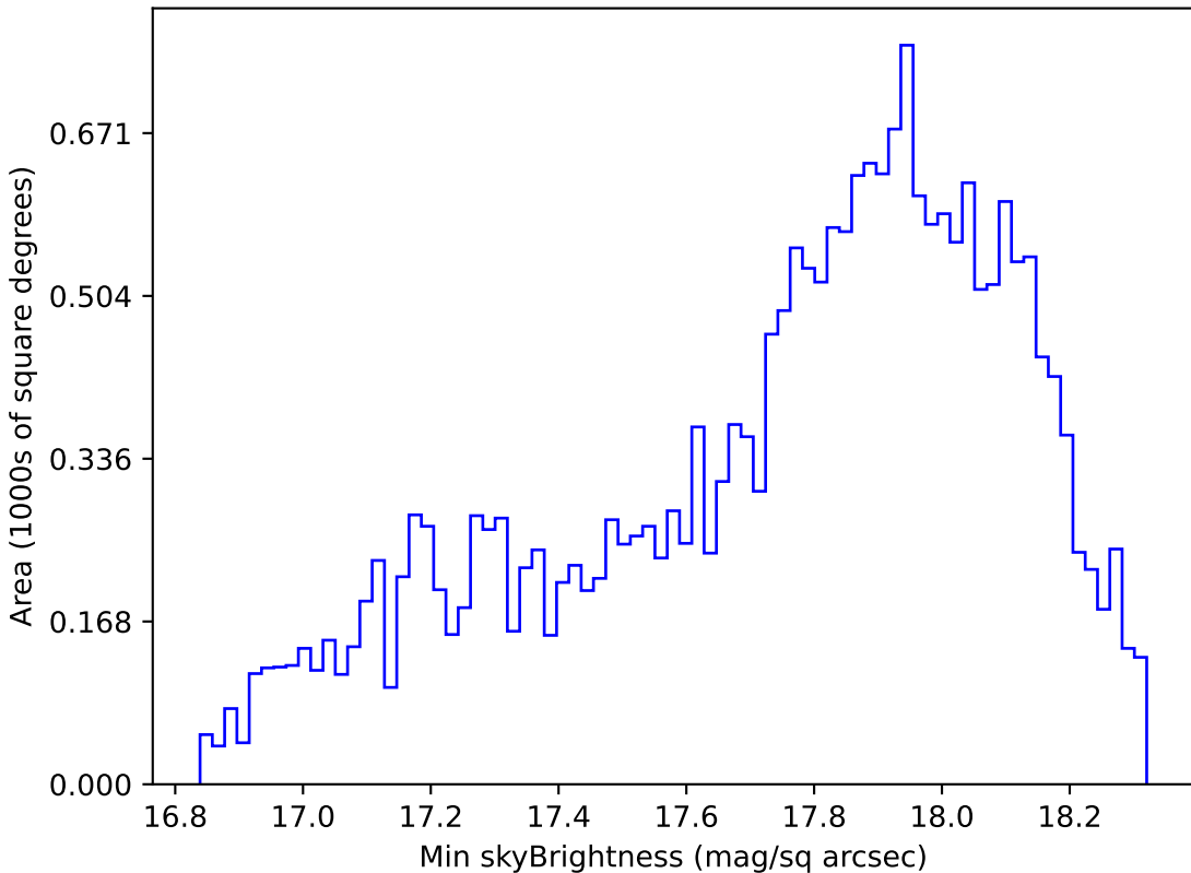
too_5_4v3.4_10yrs Yr 1 y band: Min skyBrightness
