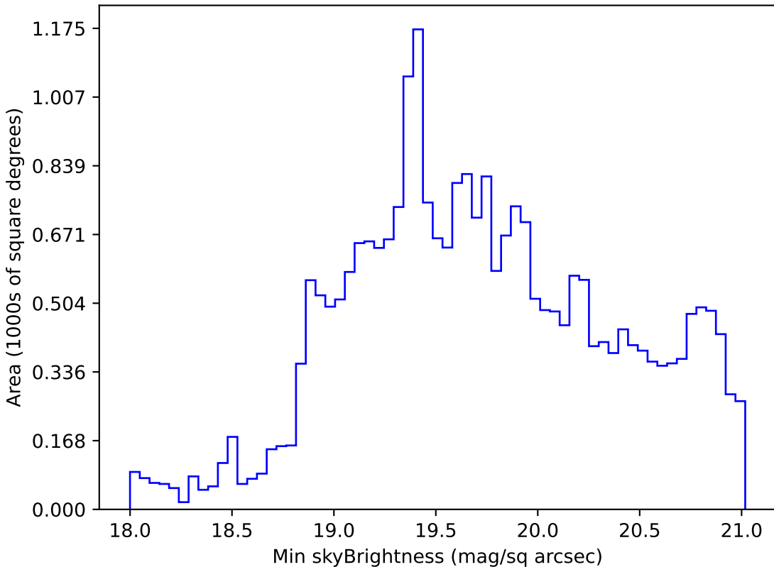
too_5_4v3.4_10yrs Yr 1 r band: Min skyBrightness
