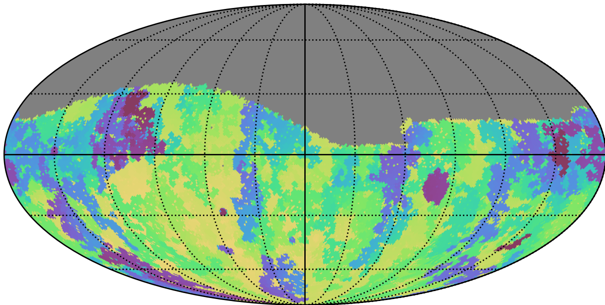
too_5_4v3.4_10yrs Yr 1 g band: Min skyBrightness
