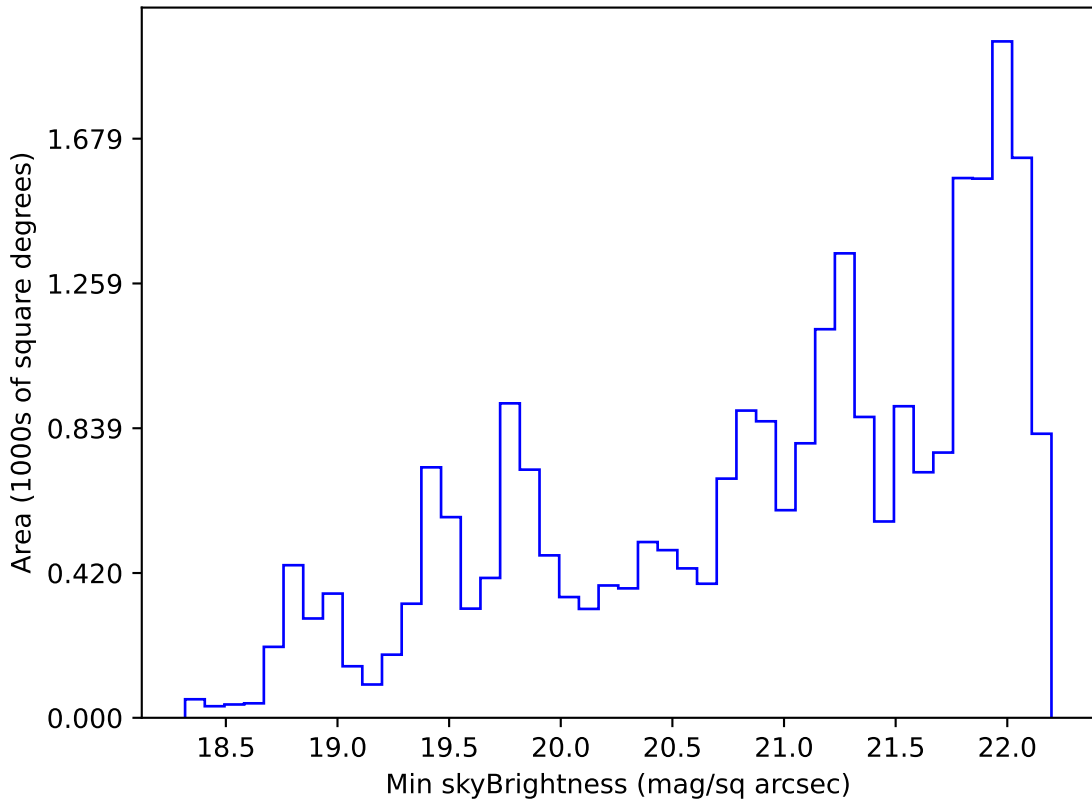
too_5_4v3.4_10yrs Yr 1 g band: Min skyBrightness
