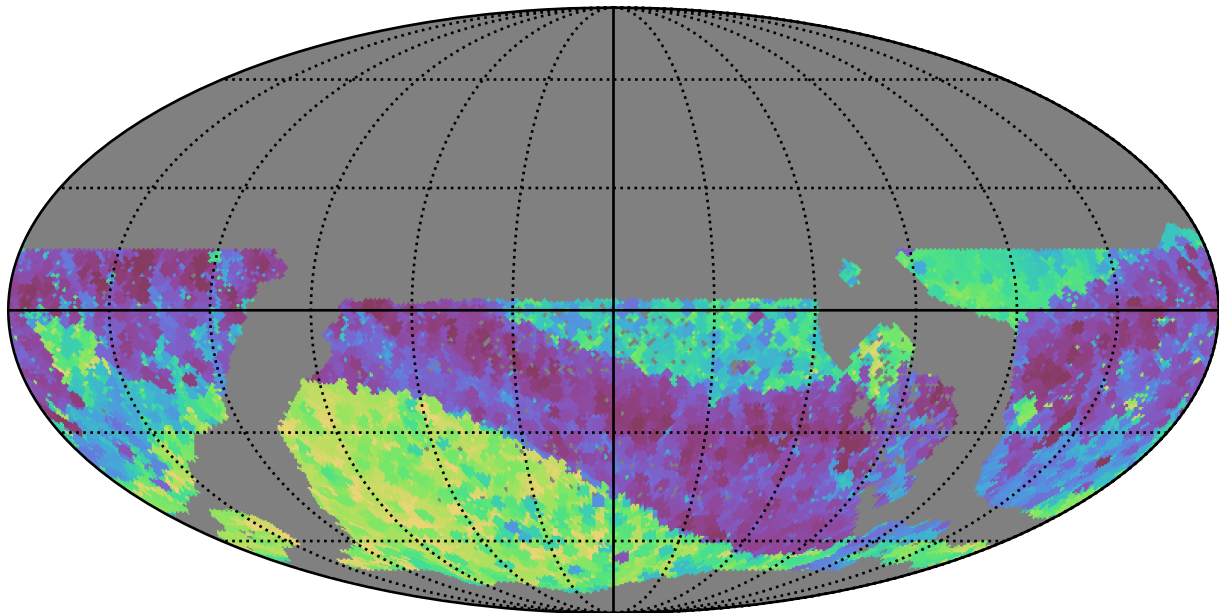
too_5_4v3.4_10yrs WFD z band: Min skyBrightness
