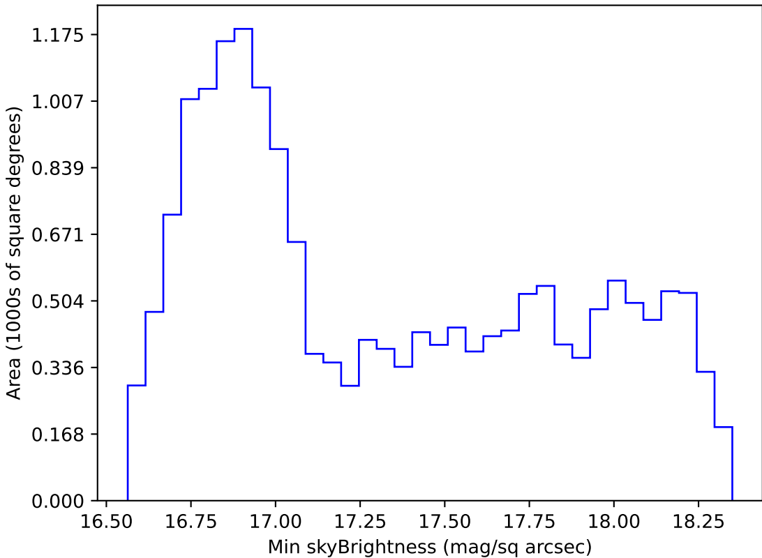
too_5_4v3.4_10yrs WFD z band: Min skyBrightness
