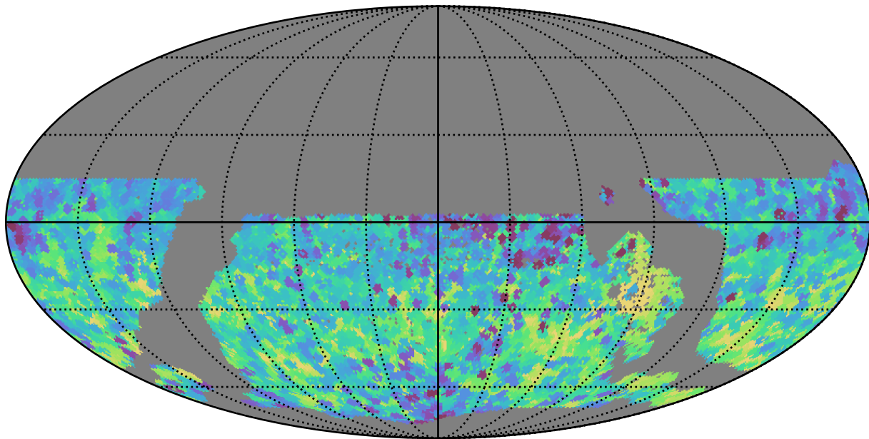
too_5_4v3.4_10yrs WFD y band: Min skyBrightness
