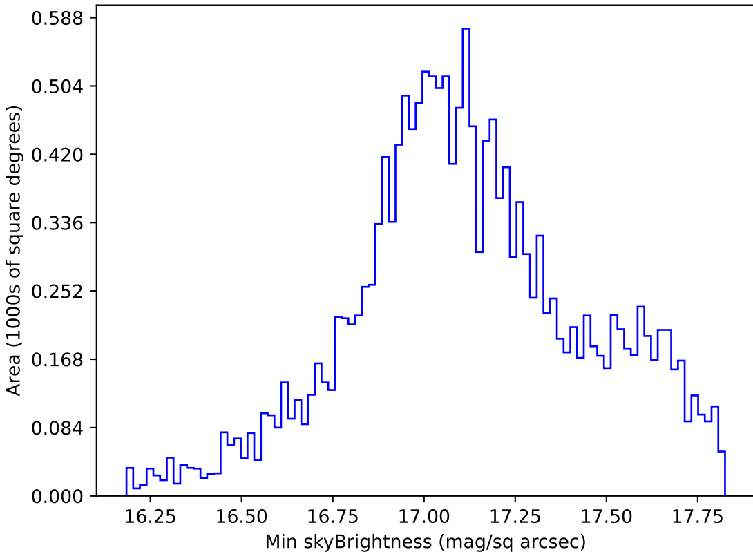
too_5_4v3.4_10yrs WFD y band: Min skyBrightness
