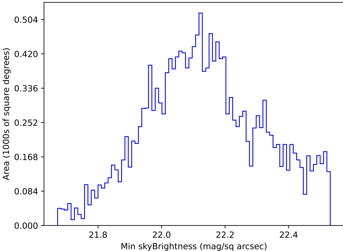
too_5_4v3.4_10yrs WFD u band: Min skyBrightness
