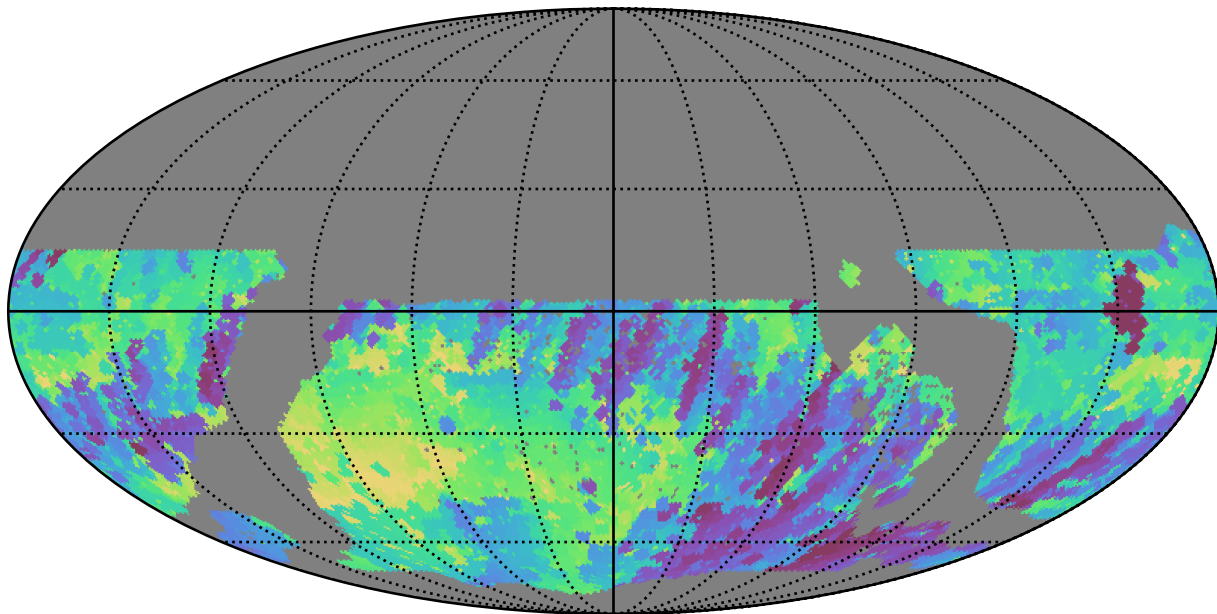
too_5_4v3.4_10yrs WFD r band: Min skyBrightness
