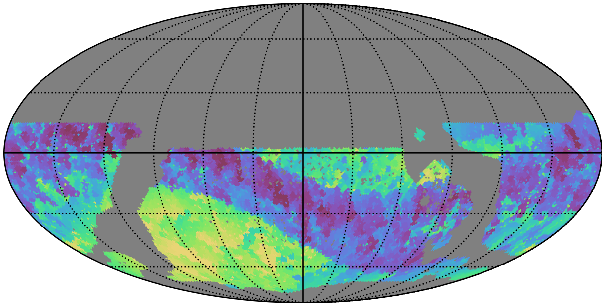
too_5_4v3.4_10yrs WFD i band: Min skyBrightness
