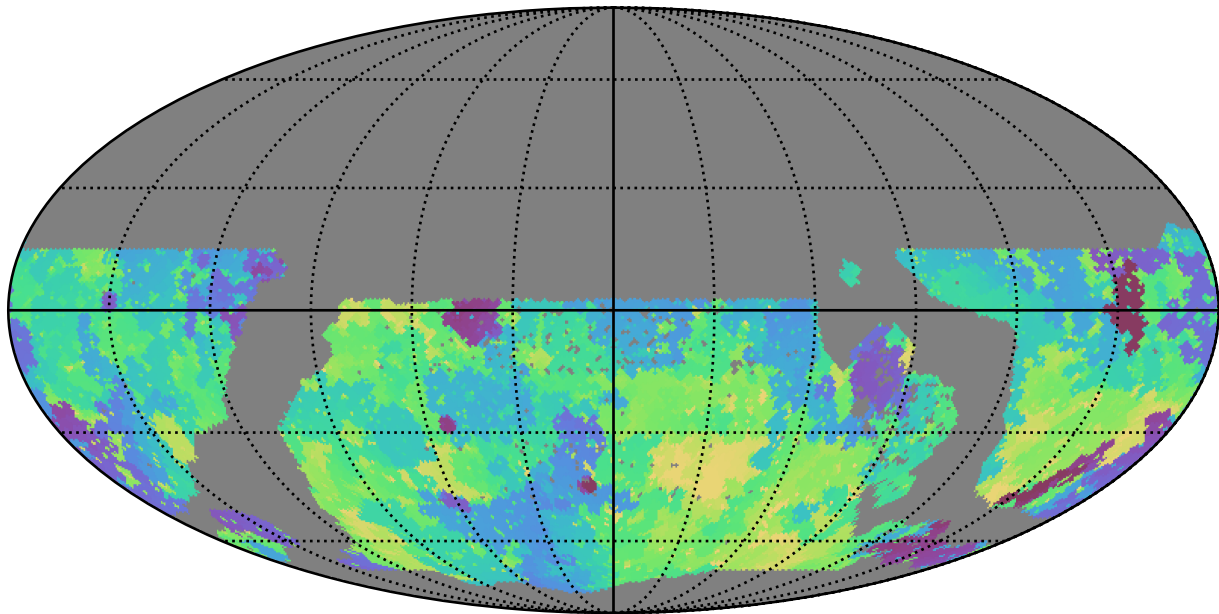
too_5_4v3.4_10yrs WFD g band: Min skyBrightness
