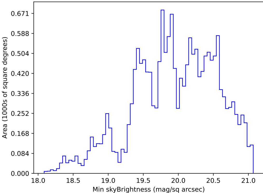
too_5_4v3.4_10yrs WFD g band: Min skyBrightness
