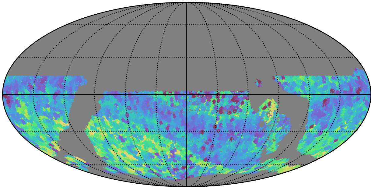
too_5_4v3.4_10yrs WFD all bands: Min skyBrightness
