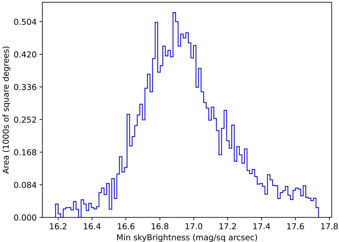
too_5_4v3.4_10yrs WFD all bands: Min skyBrightness
