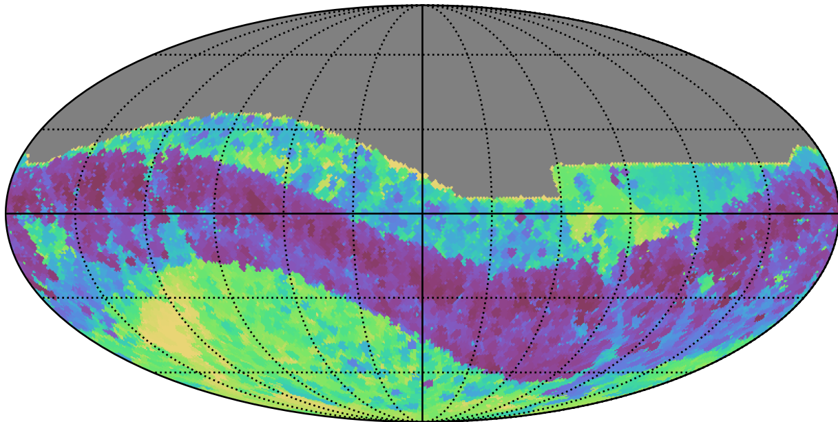
too_5_4v3.4_10yrs All sky z band: Min skyBrightness
