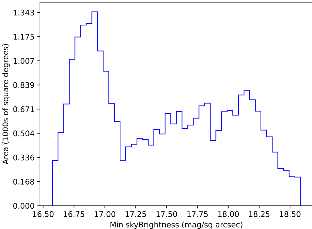
too_5_4v3.4_10yrs All sky z band: Min skyBrightness
