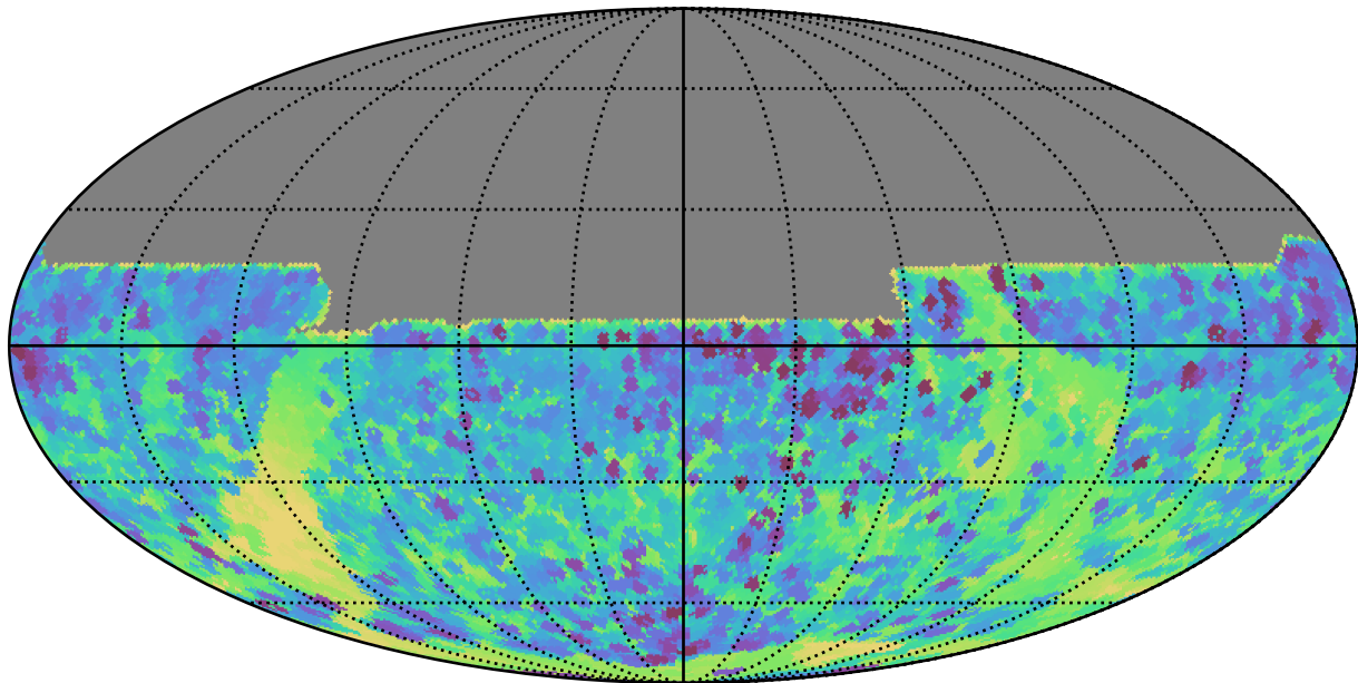
too_5_4v3.4_10yrs All sky y band: Min skyBrightness
