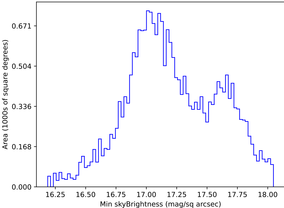
too_5_4v3.4_10yrs All sky y band: Min skyBrightness
