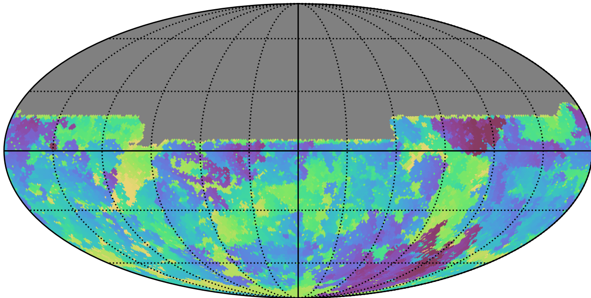
too_5_4v3.4_10yrs All sky u band: Min skyBrightness
