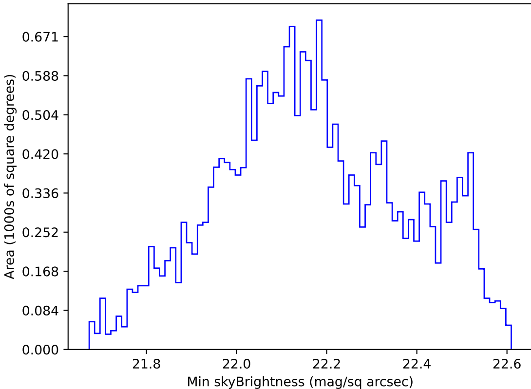
too_5_4v3.4_10yrs All sky u band: Min skyBrightness
