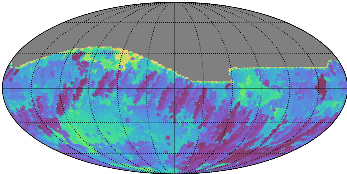
too_5_4v3.4_10yrs All sky r band: Min skyBrightness
