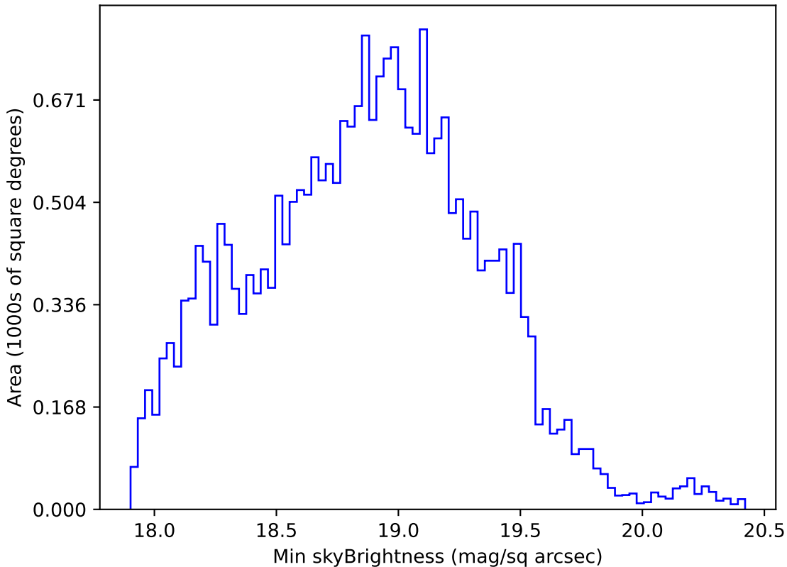
too_5_4v3.4_10yrs All sky r band: Min skyBrightness
