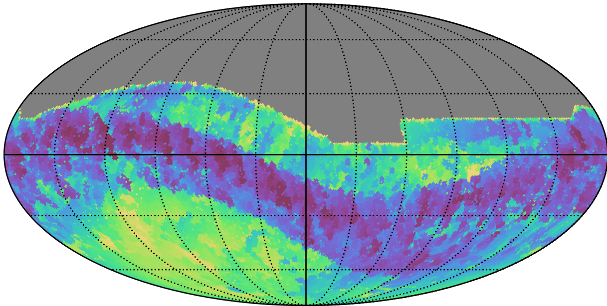
too_5_4v3.4_10yrs All sky i band: Min skyBrightness
