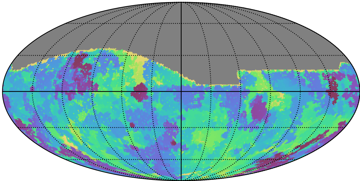
too_5_4v3.4_10yrs All sky g band: Min skyBrightness
