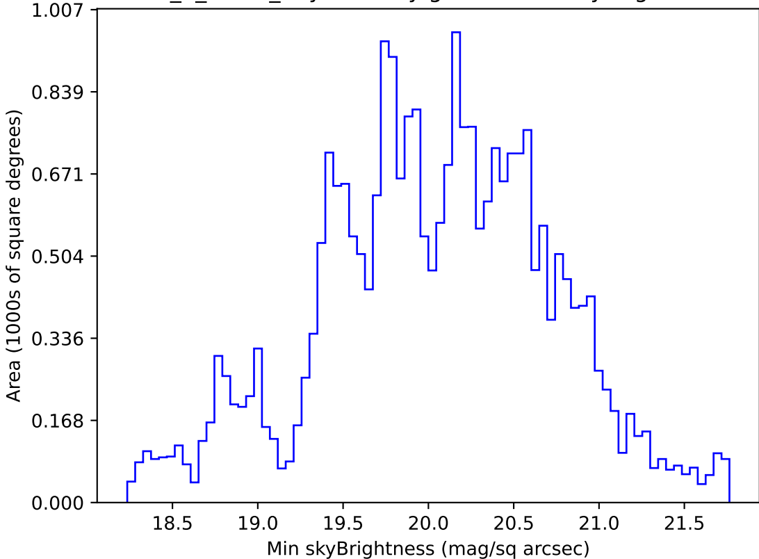
too_5_4v3.4_10yrs All sky g band: Min skyBrightness
