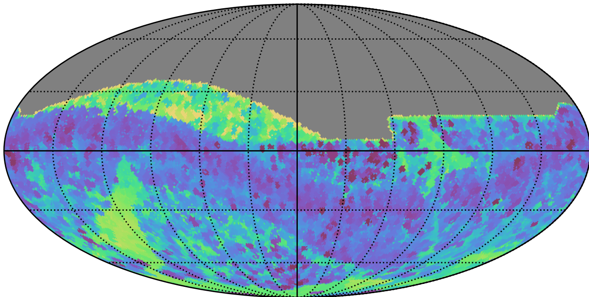
too_5_4v3.4_10yrs All sky all bands: Min skyBrightness
