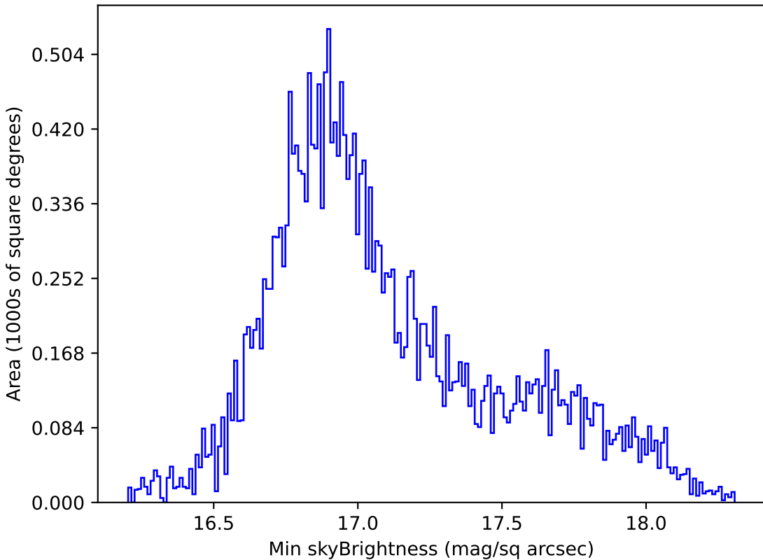
too_5_4v3.4_10yrs All sky all bands: Min skyBrightness
