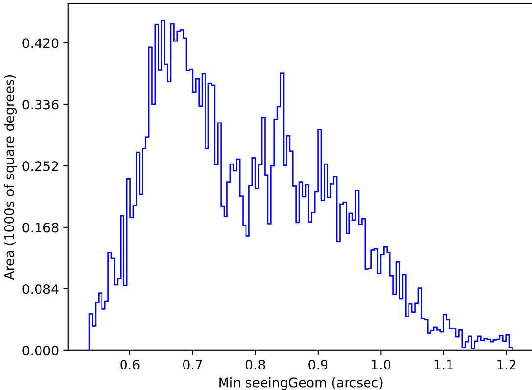
too_5_4v3.4_10yrs Yr 1 u band: Min seeingGeom
