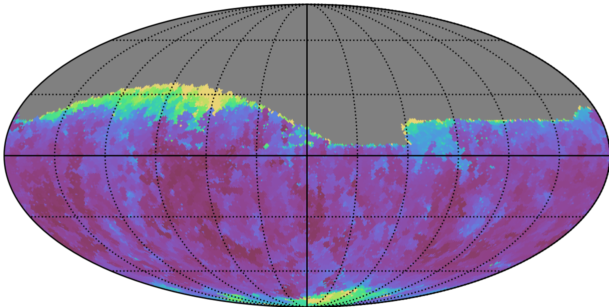
too_5_4v3.4_10yrs Yr 1 r band: Min seeingGeom
