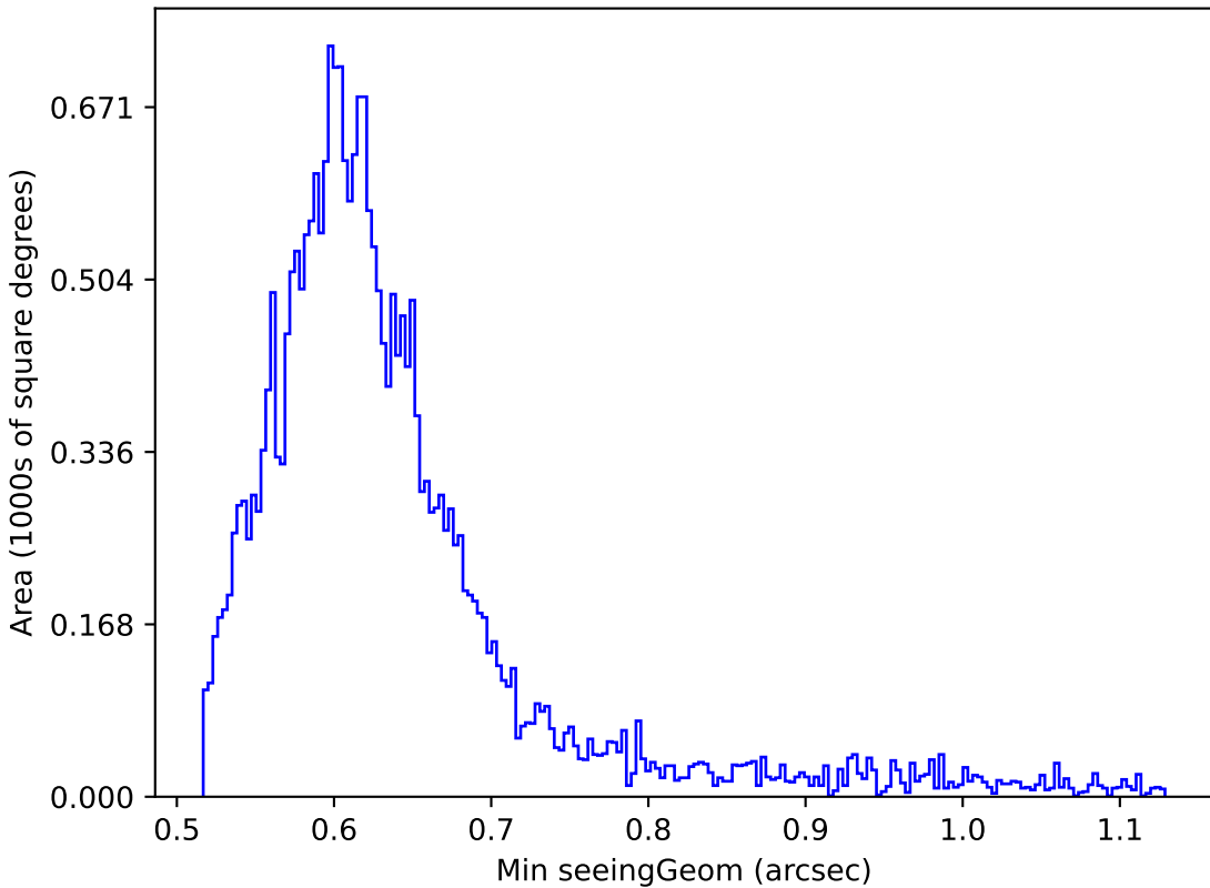
too_5_4v3.4_10yrs Yr 1 r band: Min seeingGeom
