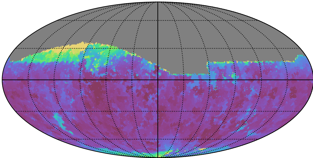
too_5_4v3.4_10yrs Yr 1 i band: Min seeingGeom
