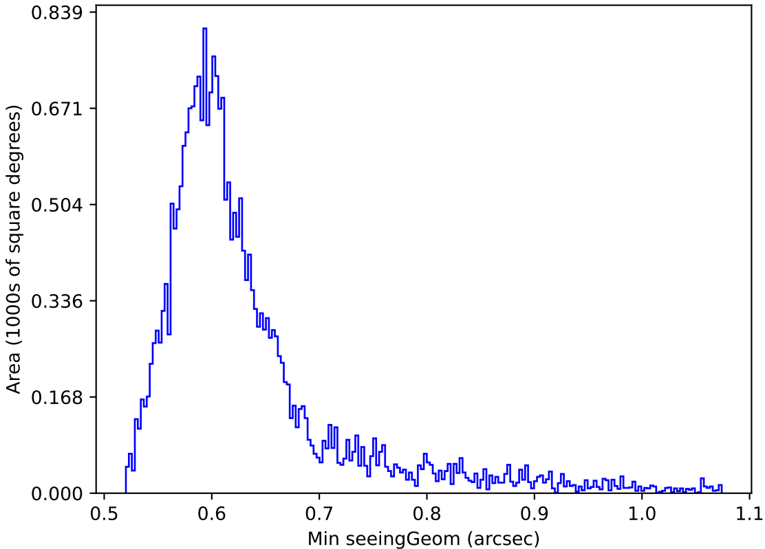
too_5_4v3.4_10yrs Yr 1 i band: Min seeingGeom
