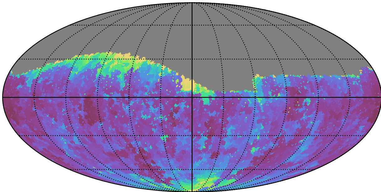
too_5_4v3.4_10yrs Yr 1 g band: Min seeingGeom
