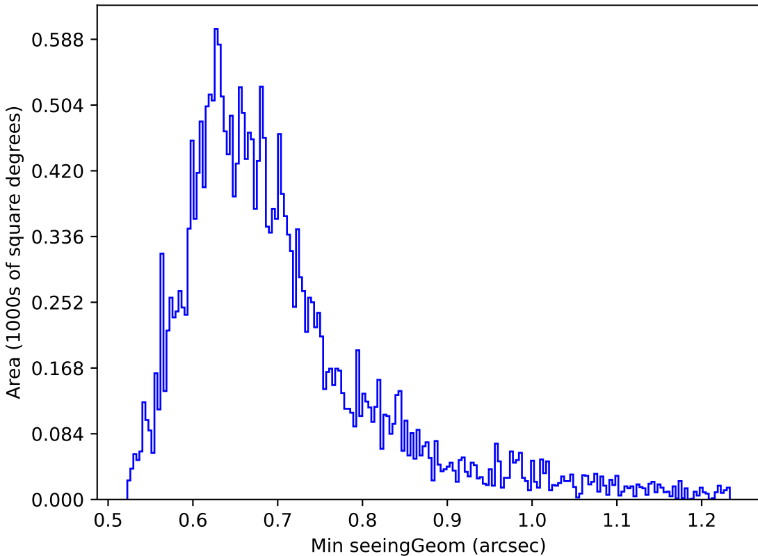
too_5_4v3.4_10yrs Yr 1 g band: Min seeingGeom
