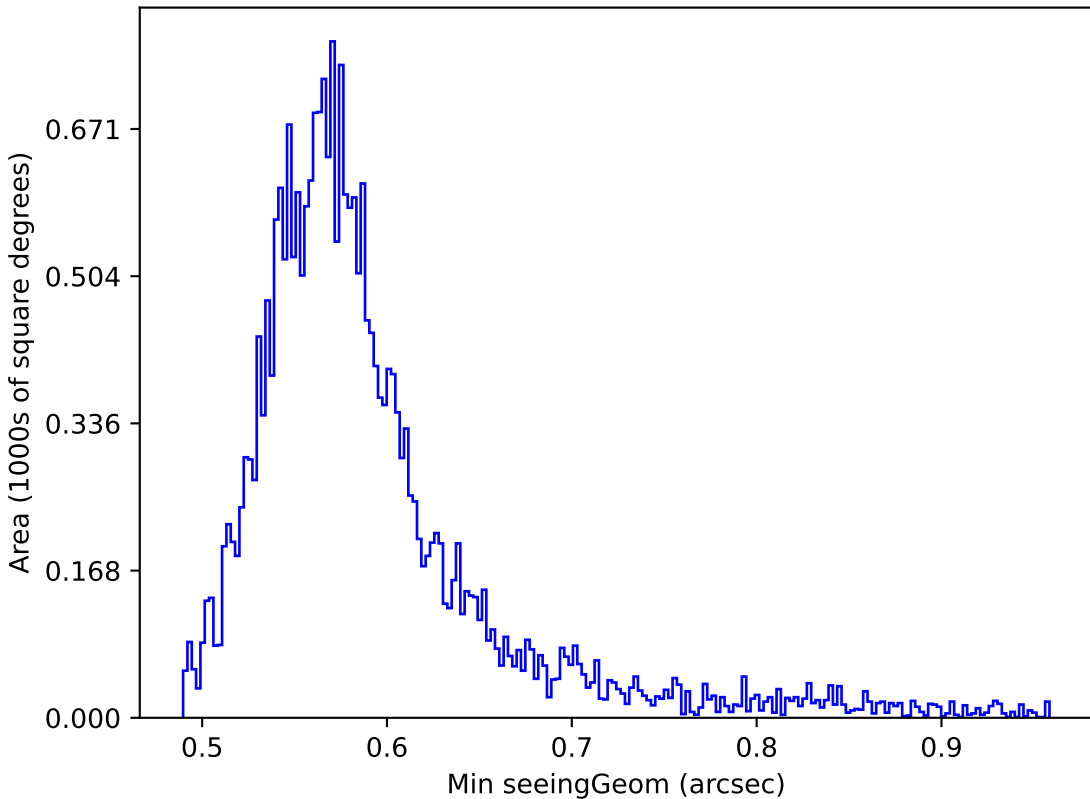
too_5_4v3.4_10yrs Yr 1 all bands: Min seeingGeom
