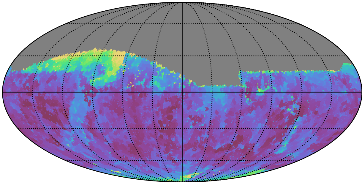
too_5_4v3.4_10yrs Yr 1 z band: Min seeingEff
