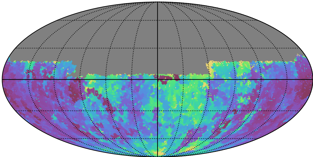
too_5_4v3.4_10yrs Yr 1 u band: Min seeingEff
