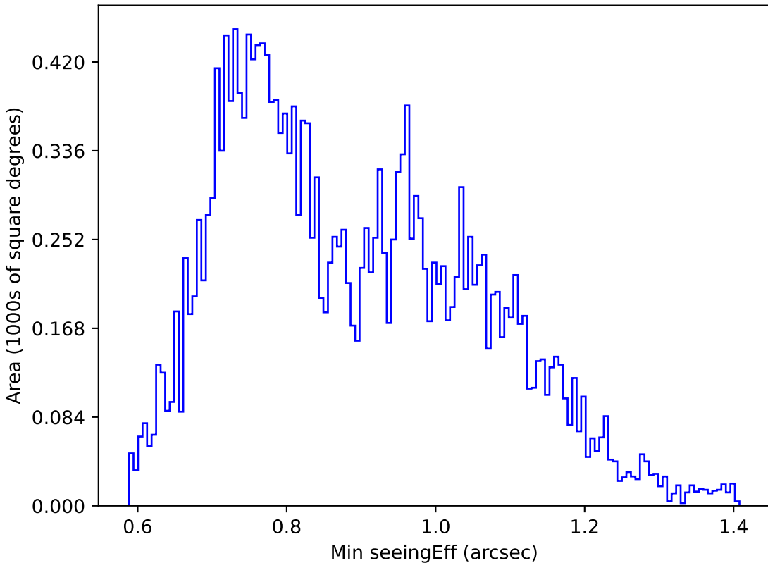
too_5_4v3.4_10yrs Yr 1 u band: Min seeingEff
