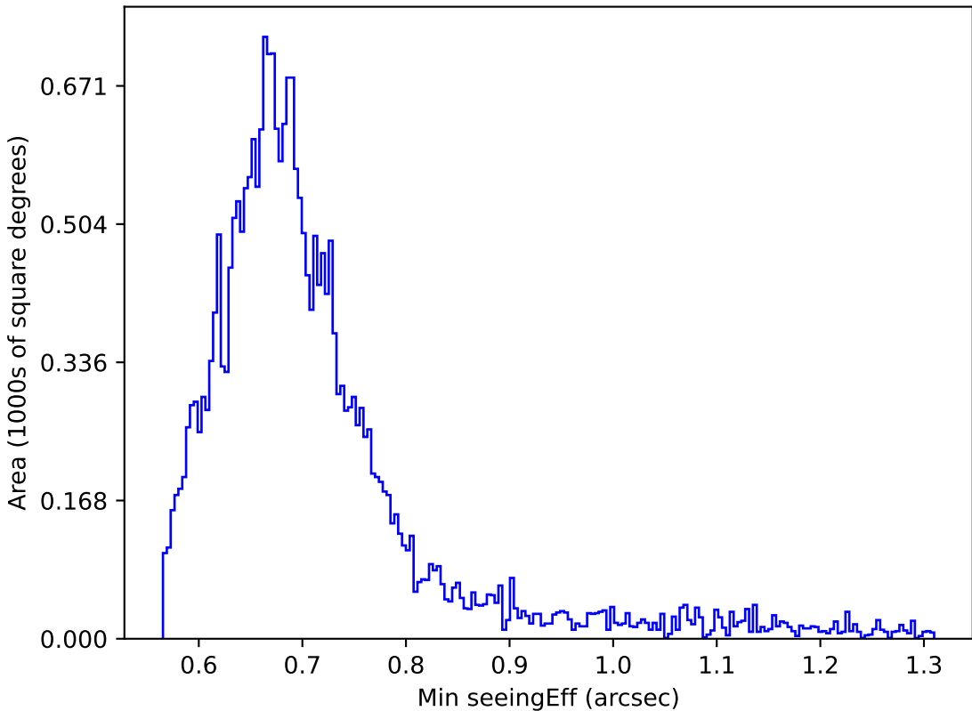
too_5_4v3.4_10yrs Yr 1 r band: Min seeingEff
